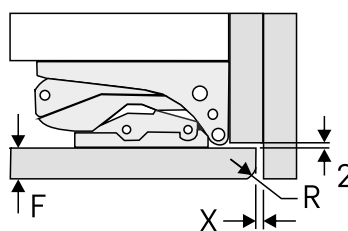
Fig. 67 Joint gap with adjoining furniture side panel
