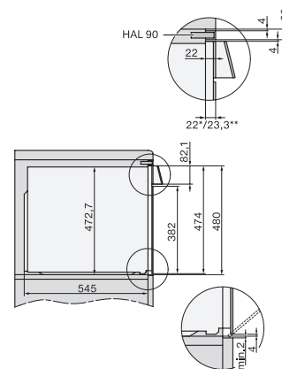
side view H7000 90 build-under, installation drawings
